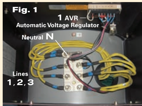
Typical AC-generator wiring connections.
