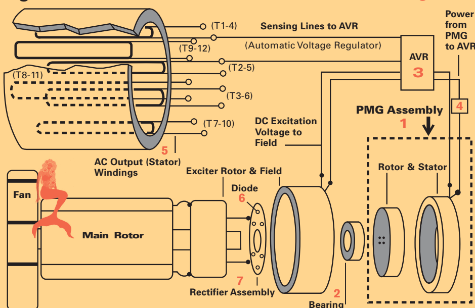
Fig. 2 PMG Generator, mounted outside the bearing.
